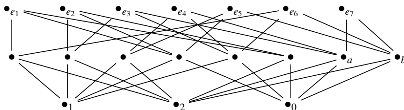
Figure 4.2: The face poset of H \cup e_7 .
