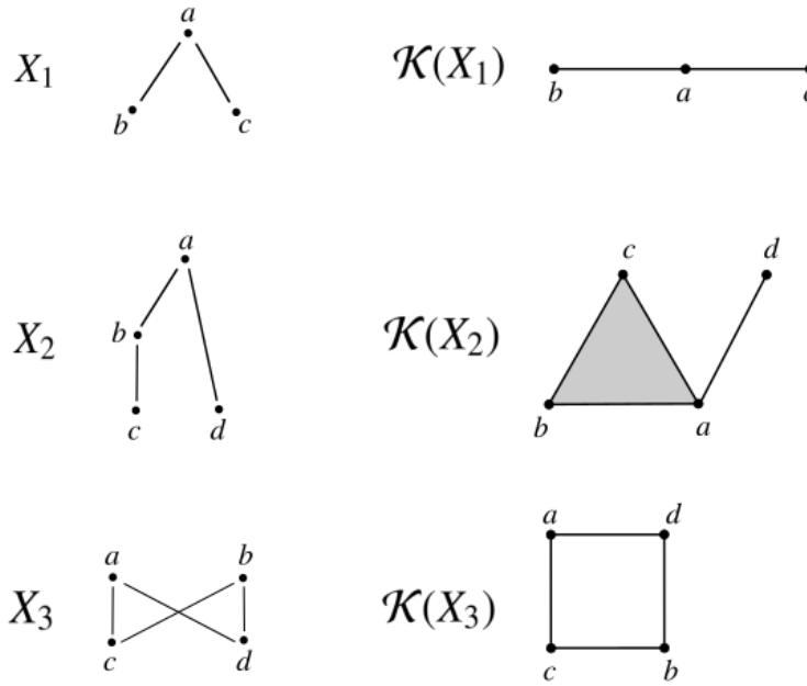
Figure 2.2: Order complexes of some finite topological spaces.
