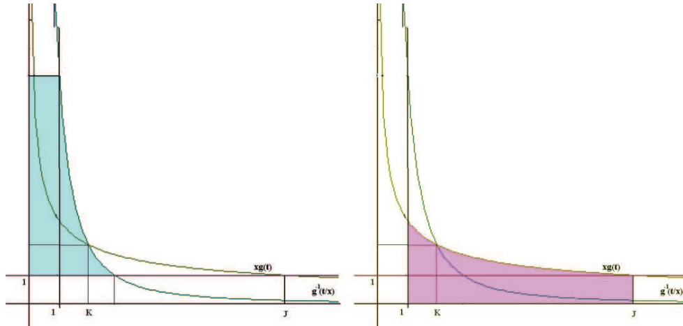
Figure 3.1: Symmetry argument in the proof.
